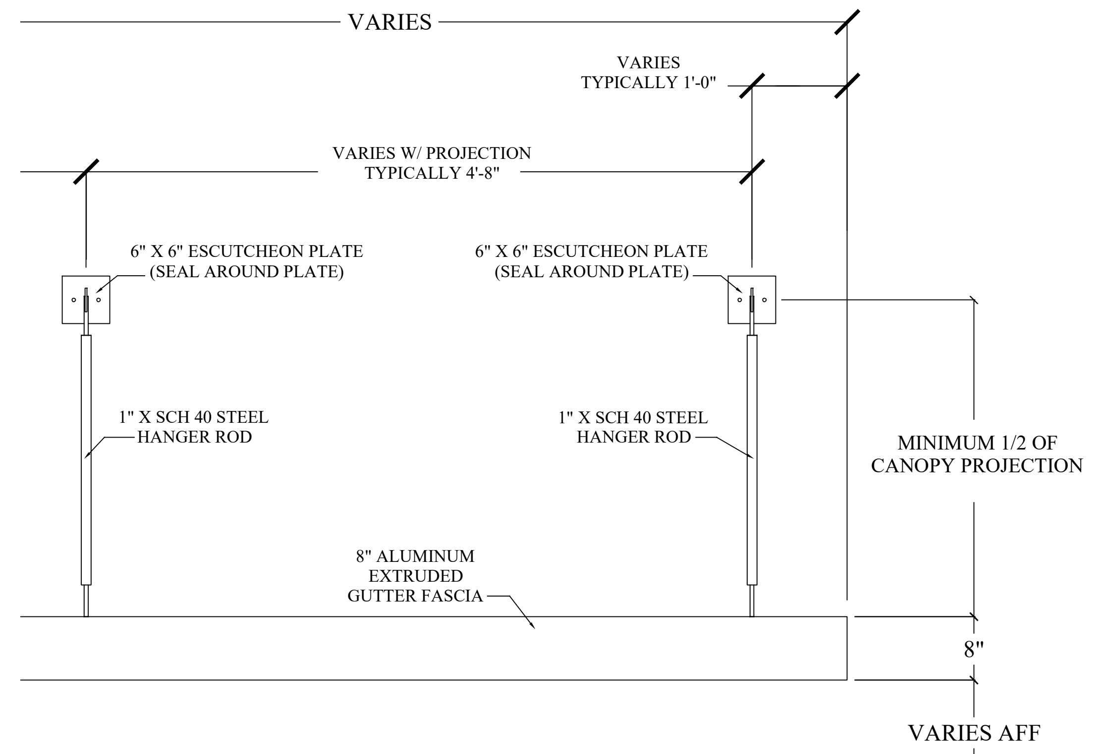
? ELEVATION VIEW - HANGER ROD CANOPY ???. SCALE: 1" = 1'
