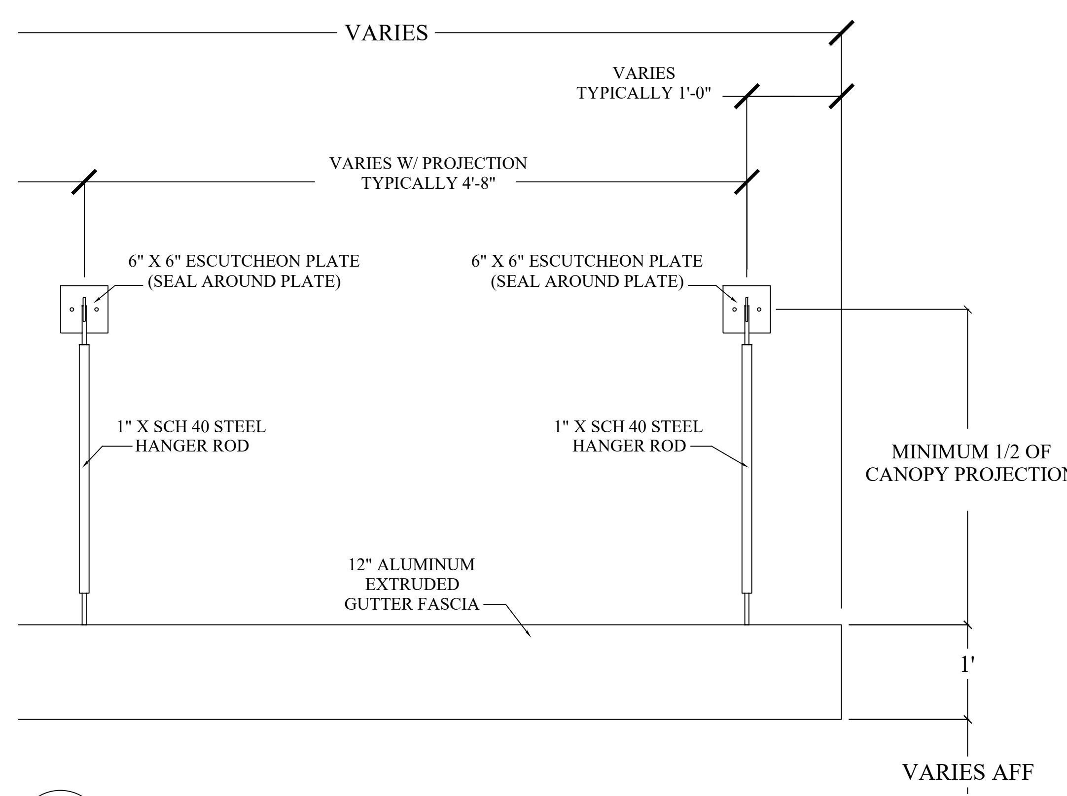
? ELEVATION VIEW - HANGER ROD CANOPY ??? SCALE: 1" = 1'
